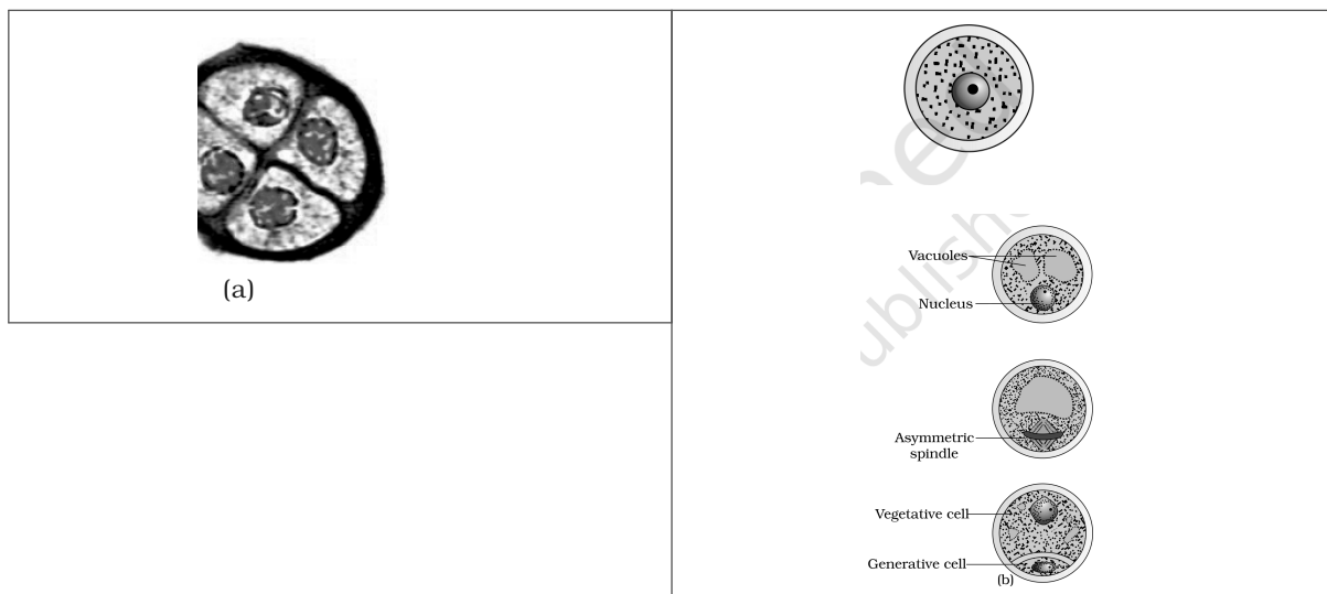
Fig. 1.5 — (a) Enlarged view of a pollen grain tetrad; (b) stages of a microspore maturing into a pollen grain. Labelled: vacuoles, nucleus, asymmetric spindle, vegetative cell, generative cell.
