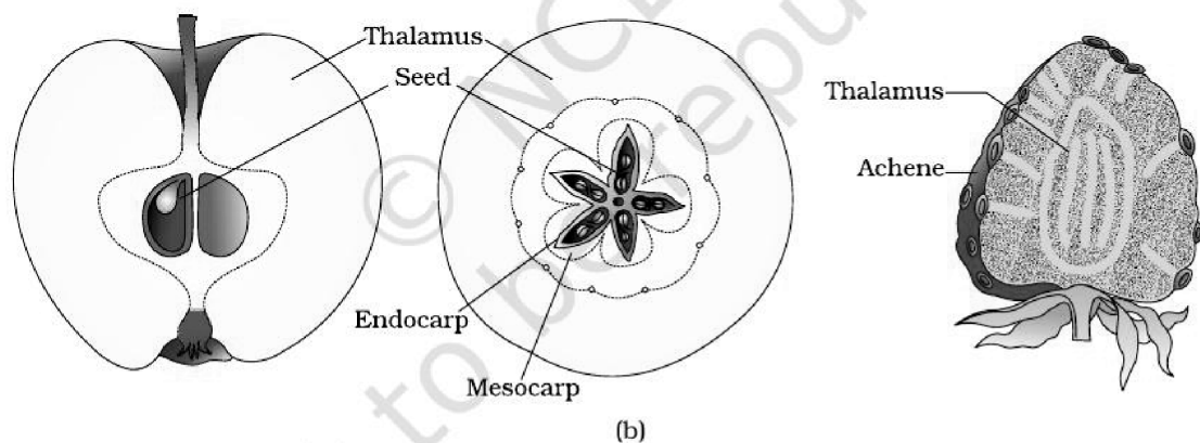
Fig. 1.15 — (a) Structure of some seeds. (b) False fruits of apple and strawberry. Labelled: cotyledons, micropyle, seed coat, endosperm, hypocotyl root axis, shoot apical meristem, root tip, scutellum, coleoptile, plumule, radicle, coleorhiza, pericarp, thalamus, seed, endocarp, mesocarp, achene.
